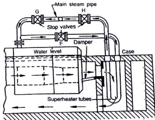
Fig. Superheater
